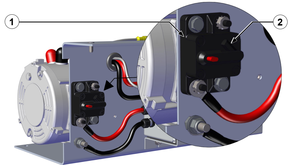
1. Foam pump 2. Inject/discharge valve
