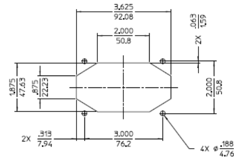
PANEL CUT-OUT
