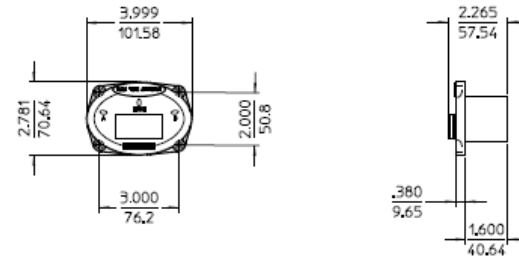
CONTROLLER
