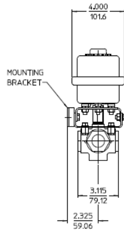
ELECTRIC VALVE
