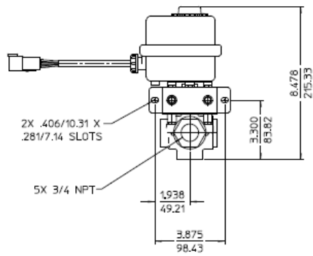
ELECTRIC VALVE
