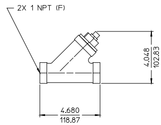
STRAINER (3) FURNISHED
