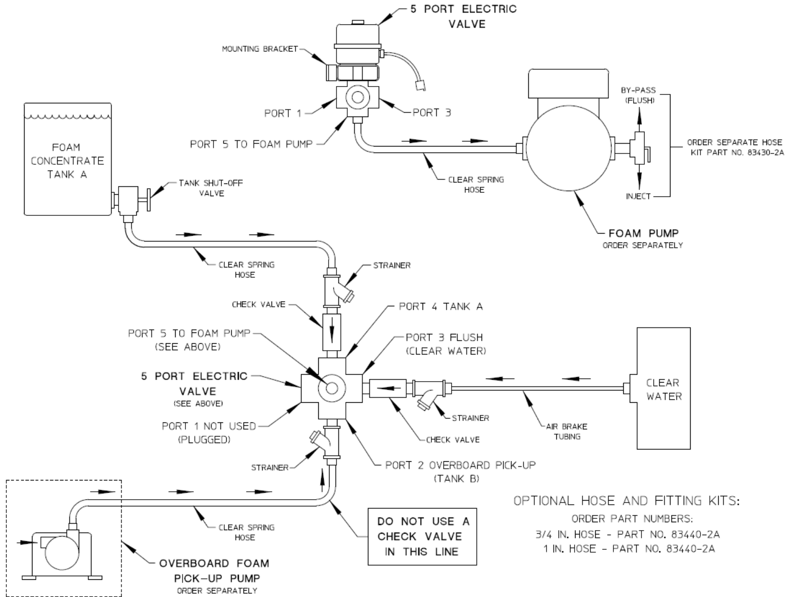
PLUMBING ONE TANK AND OVERBOARD PICK-UP CONFIGURATION
