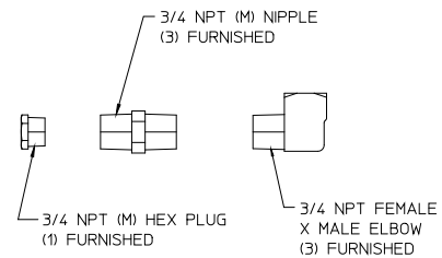
FITTING KIT
