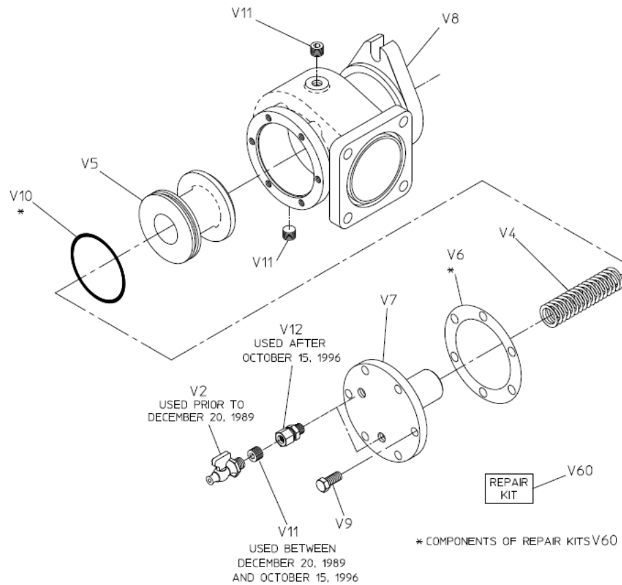
LEFT FACING DISCHARGE ASSEMBLY 80397-3 AND 80397-4
