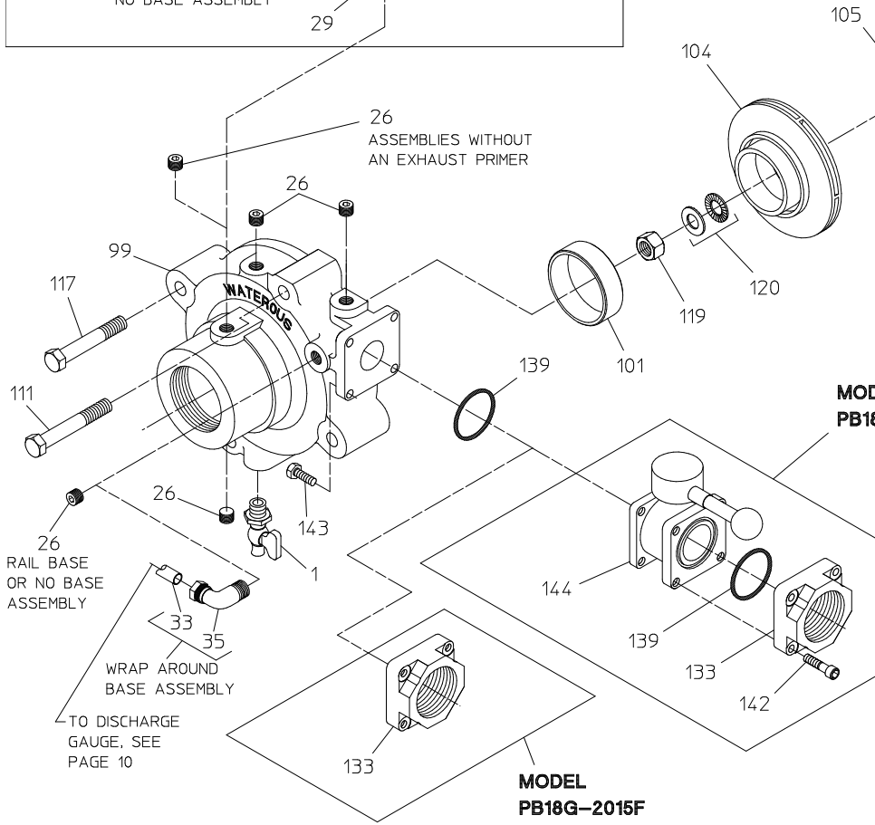
PUMP ASSEMBLY FOR MODELS PB18G-2015B & PB18G-2015F (SEE PAGE 4 FOR PUMP ASSEMBLY CROSS SECTION VIEW)
