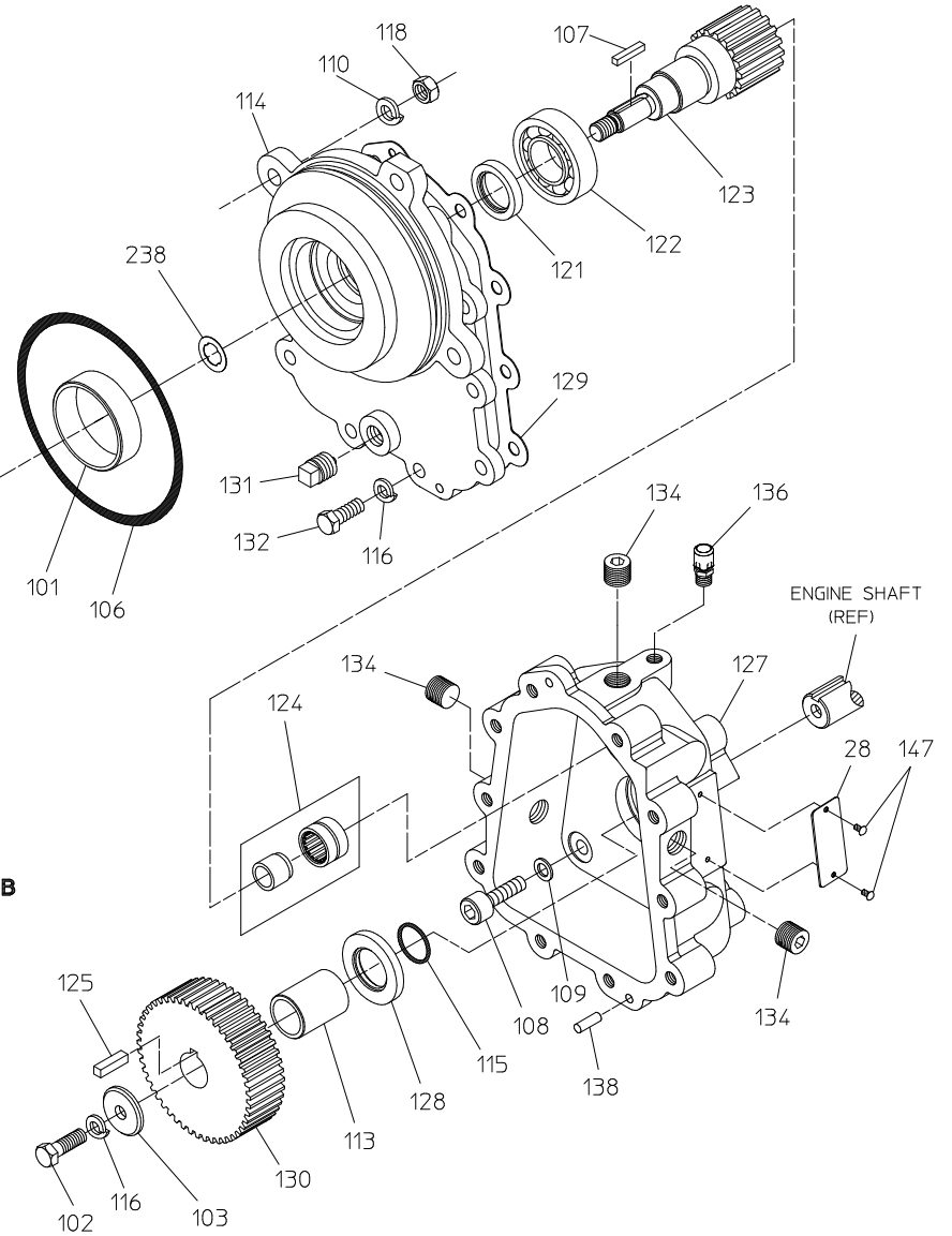
PUMP ASSEMBLY FOR MODELS PB18G-2015B & PB18G-2015F (SEE PAGE 4 FOR PUMP ASSEMBLY CROSS SECTION VIEW)
