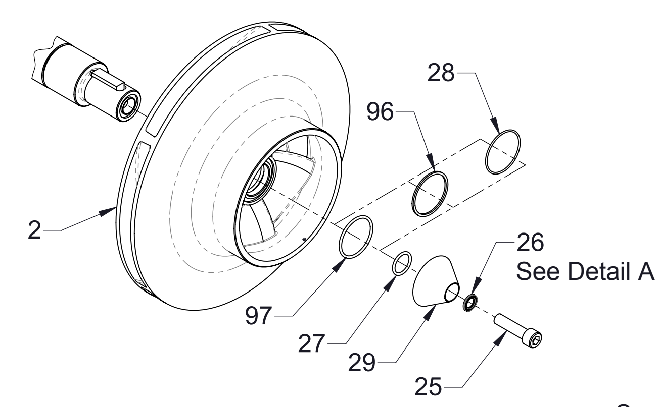
Impeller Cone Design (Used prior to February 1, 2020)
