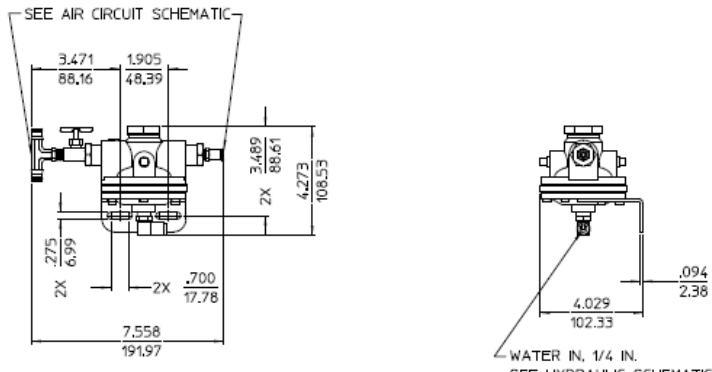
BALANCE VALVE
