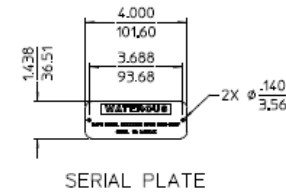
SERIAL PLATE
